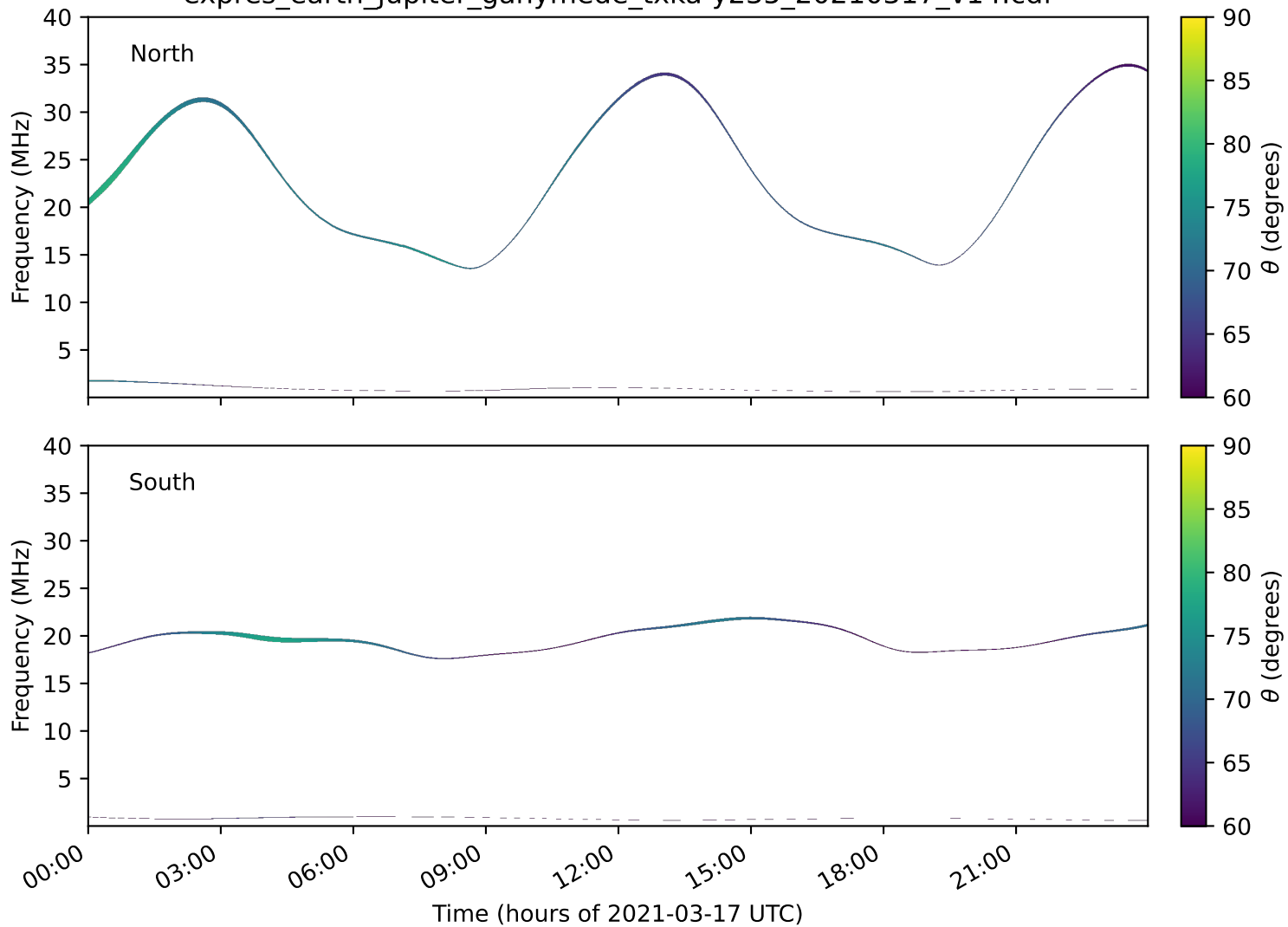
expres_earth_jupiter_ganymede_txka-y235_20210317_v14.cdf
