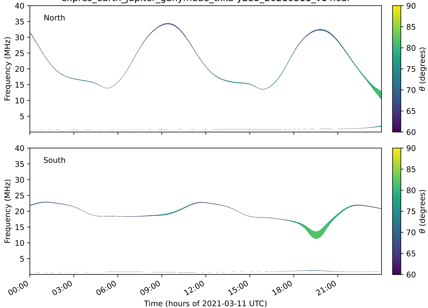
expres_earth_jupiter_ganymede_txka-y235_20210311_v14.cdf
