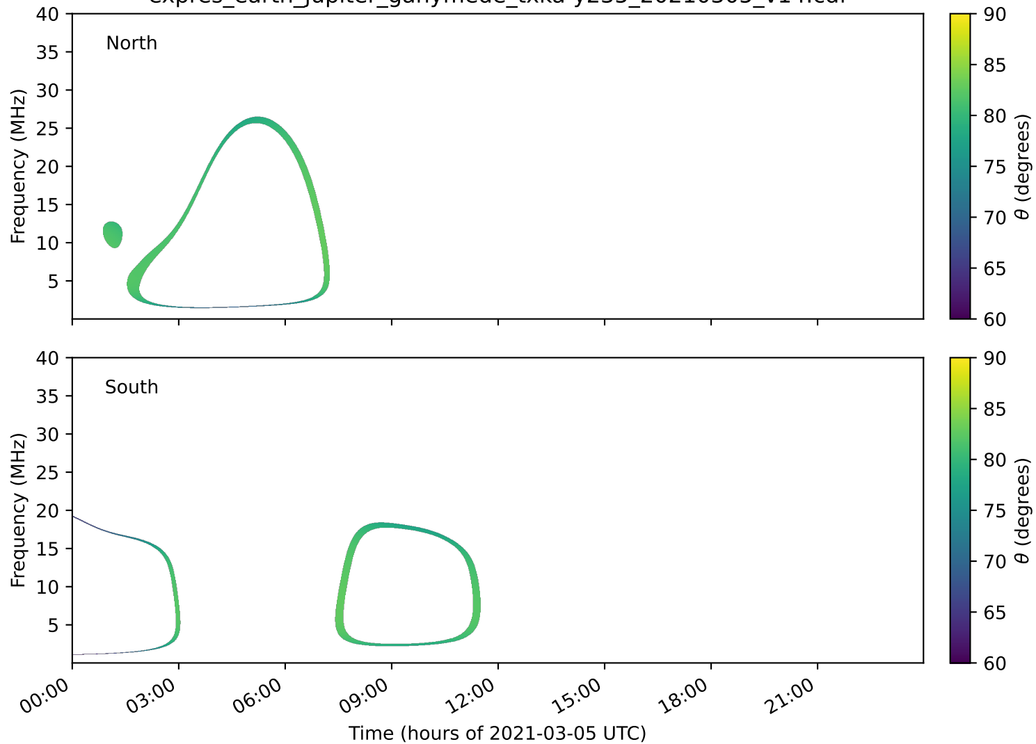
expres_earth_jupiter_ganymede_txka-y235_20210305_v14.cdf
