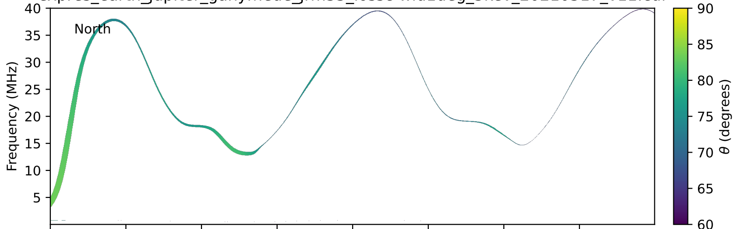
expres_earth_jupiter_ganymede_jrm33_lossc-wid1deg_3kev_20210317_v11.cdf
