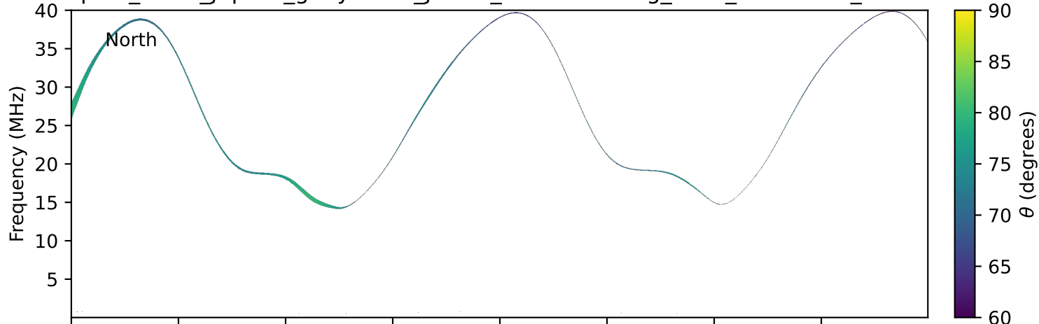
expres_earth_jupiter_ganymede_jrm33_lossc-wid1deg_3kev_20210310_v11.cdf
