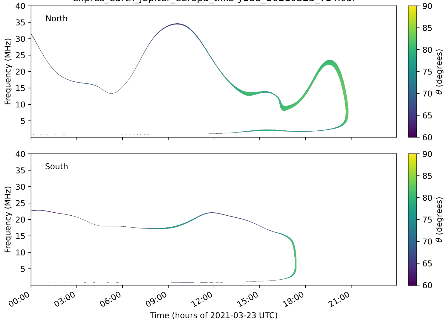
expres_earth_jupiter_europa_txka-y235_20210323_v14.cdf
