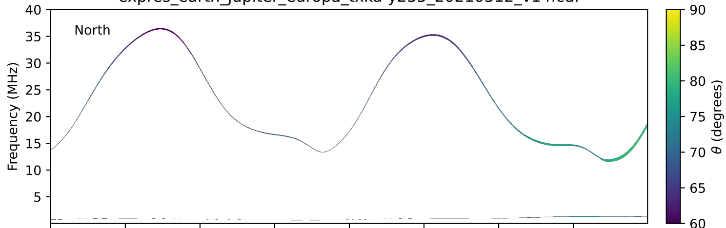
expres_earth_jupiter_europa_txka-y235_20210312_v14.cdf
