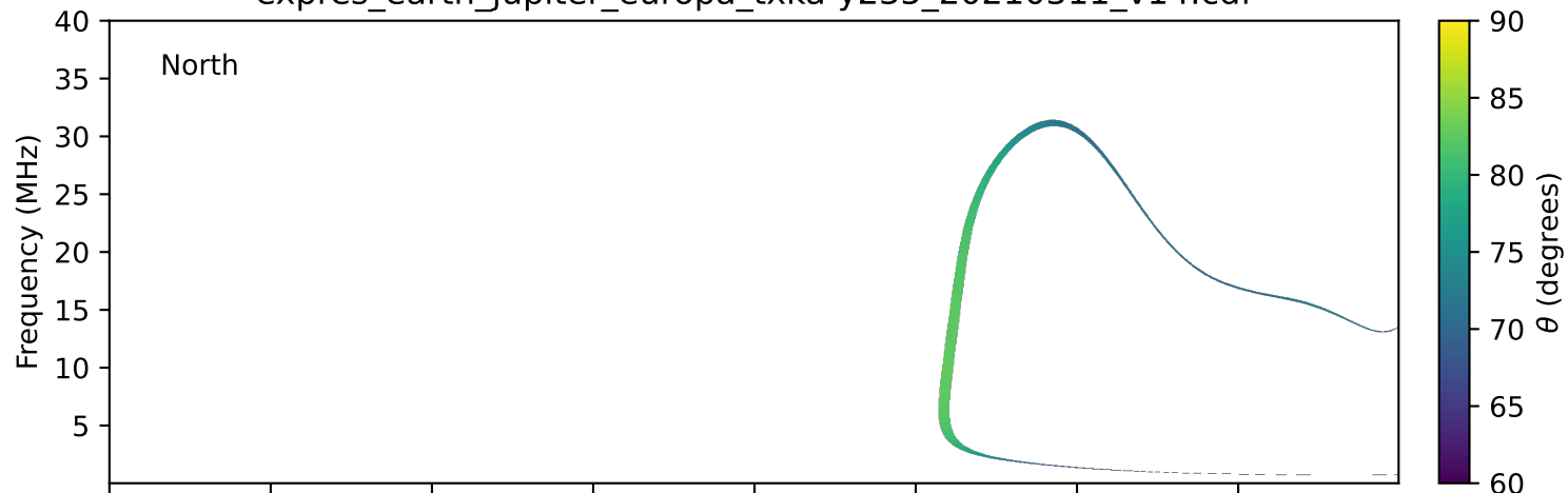
expres_earth_jupiter_europa_txka-y235_20210311_v14.cdf
