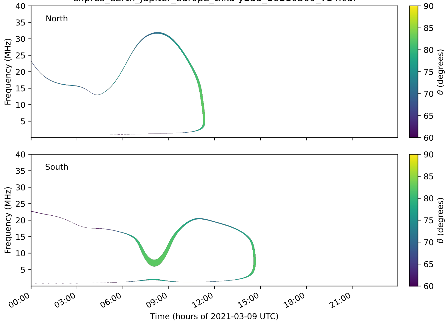
expres_earth_jupiter_europa_txka-y235_20210309_v14.cdf
