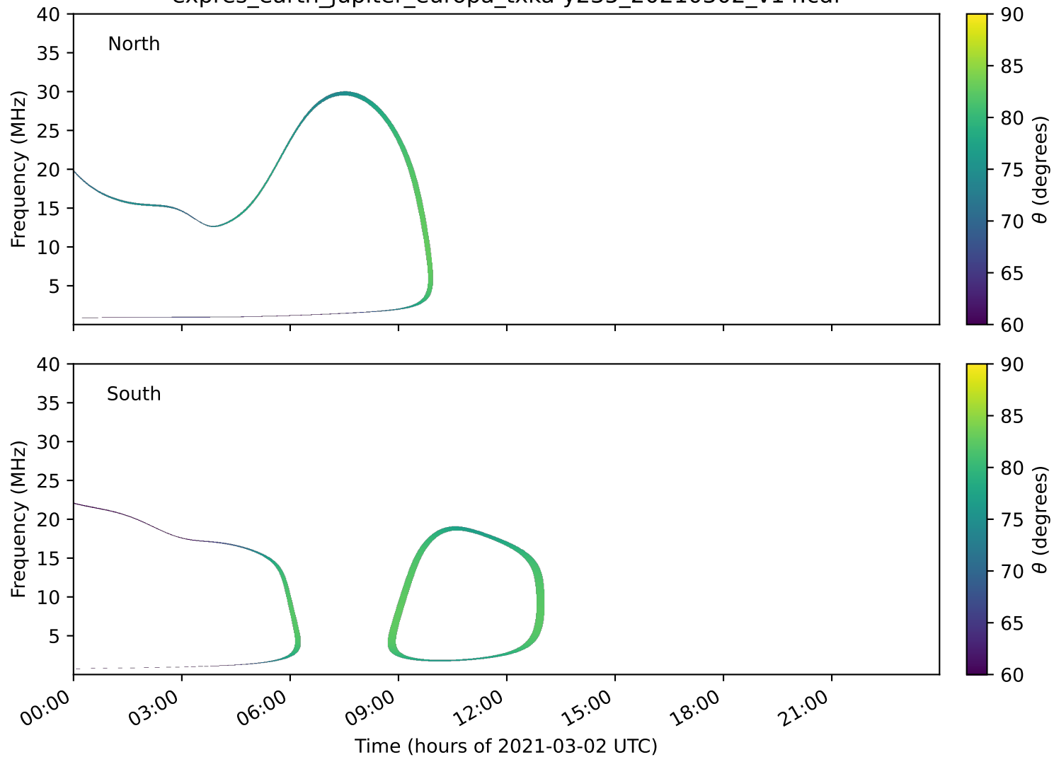
expres_earth_jupiter_europa_txka-y235_20210302_v14.cdf
