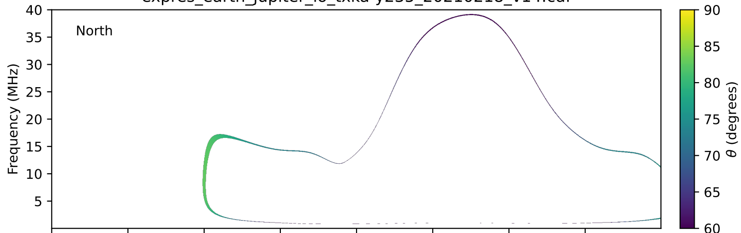
expres_earth_jupiter_io_txka-y235_20210218_v14.cdf
