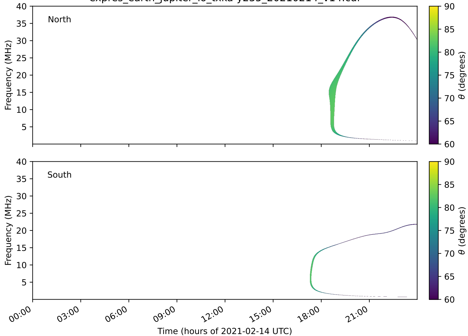
expres_earth_jupiter_io_txka-y235_20210214_v14.cdf
