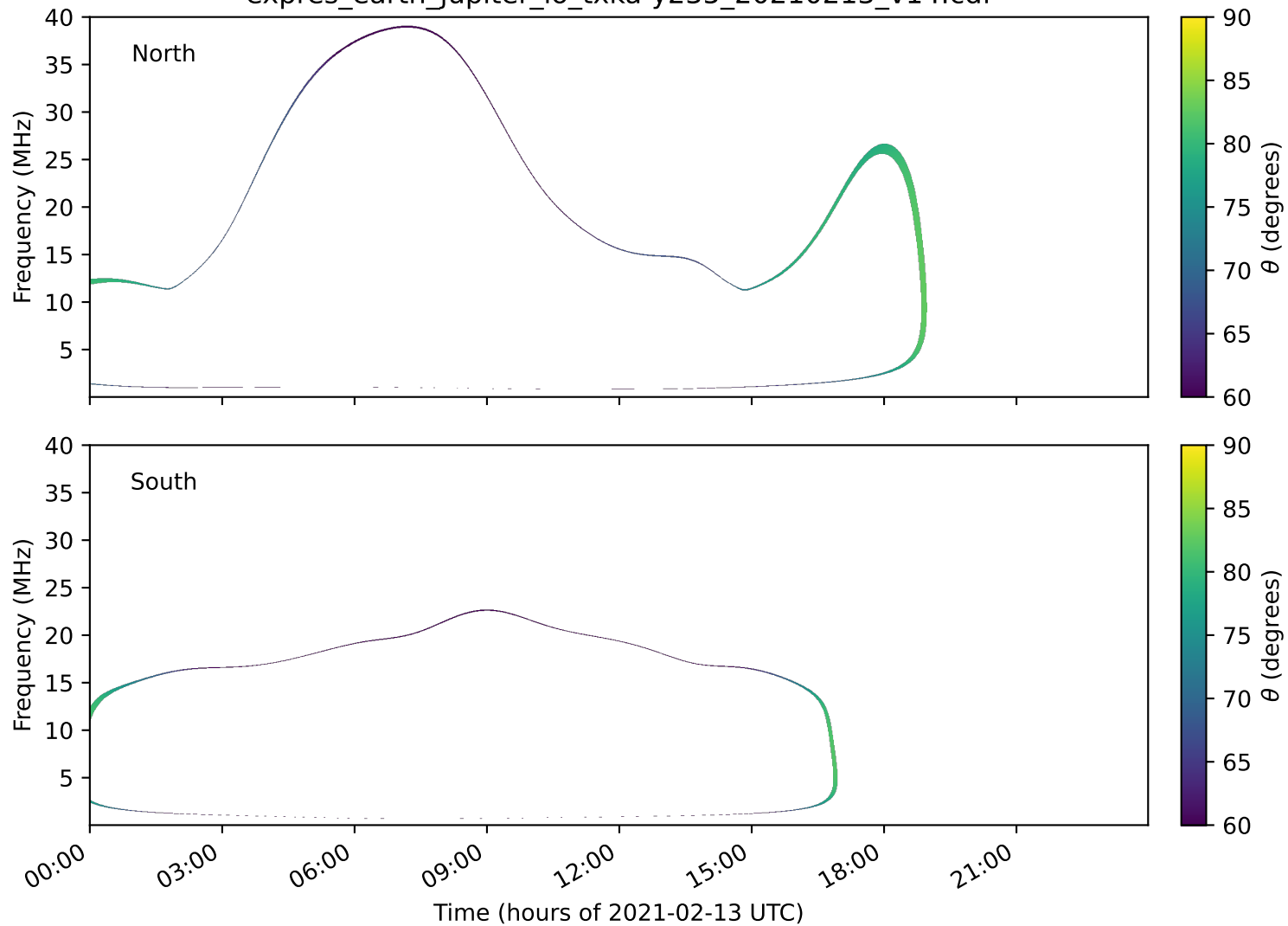
expres_earth_jupiter_io_txka-y235_20210213_v14.cdf
