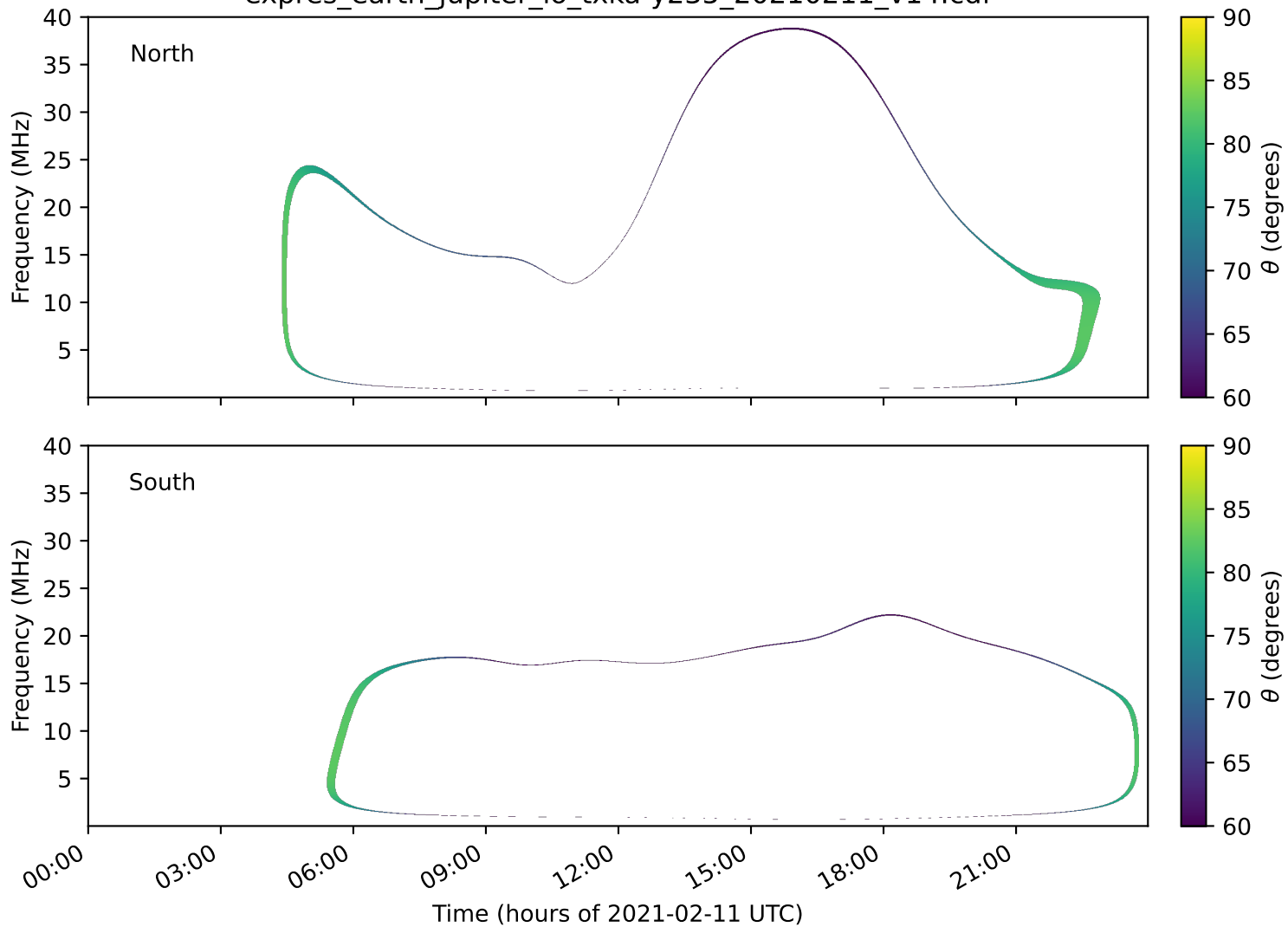
expres_earth_jupiter_io_txka-y235_20210211_v14.cdf
