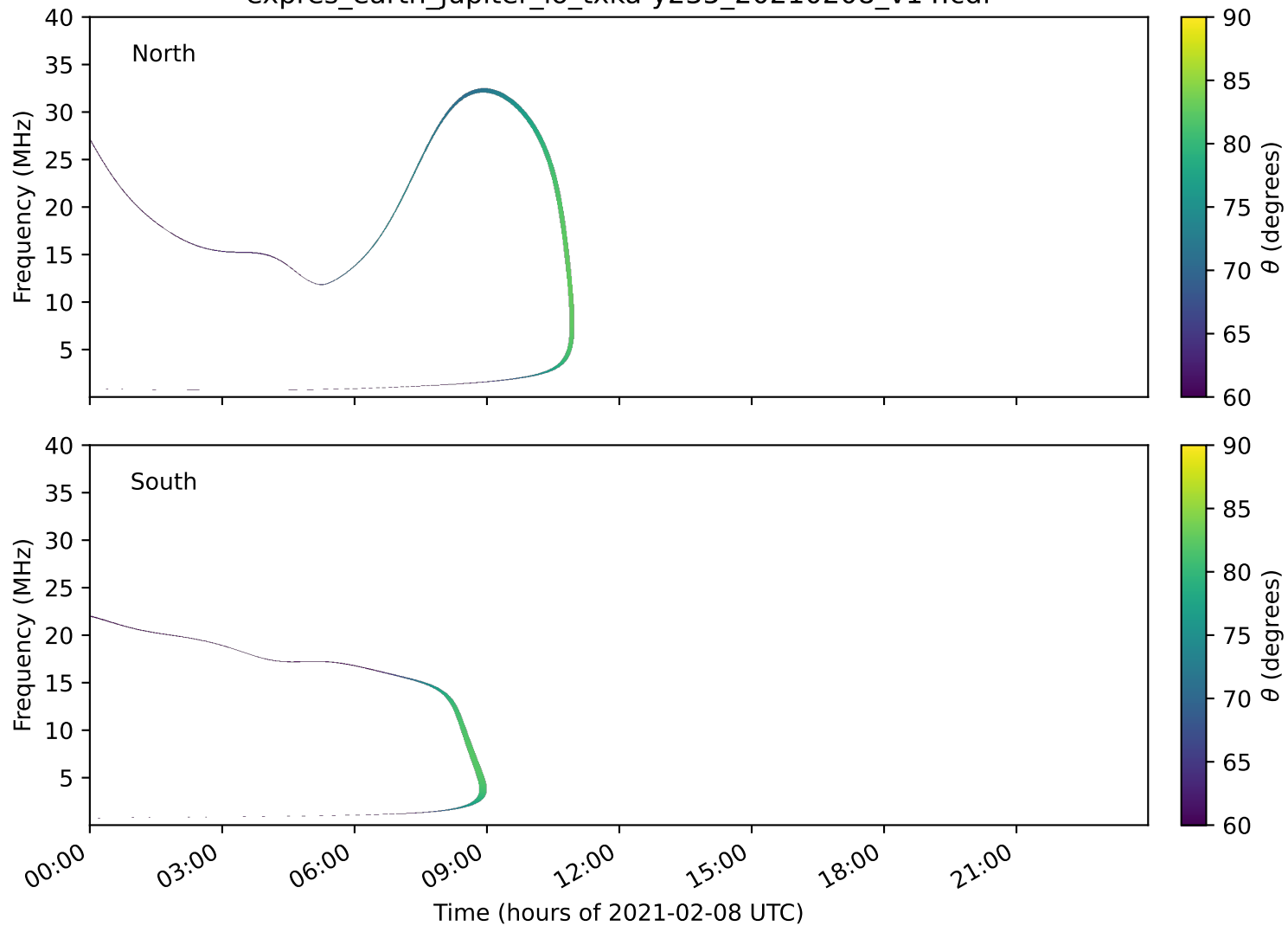
expres_earth_jupiter_io_txka-y235_20210208_v14.cdf
