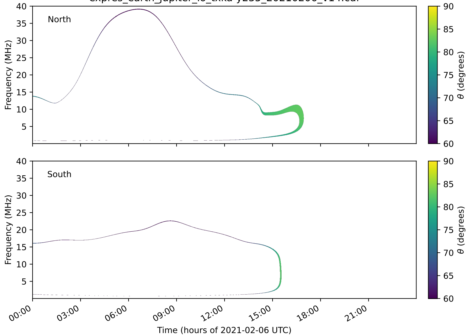
expres_earth_jupiter_io_txka-y235_20210206_v14.cdf
