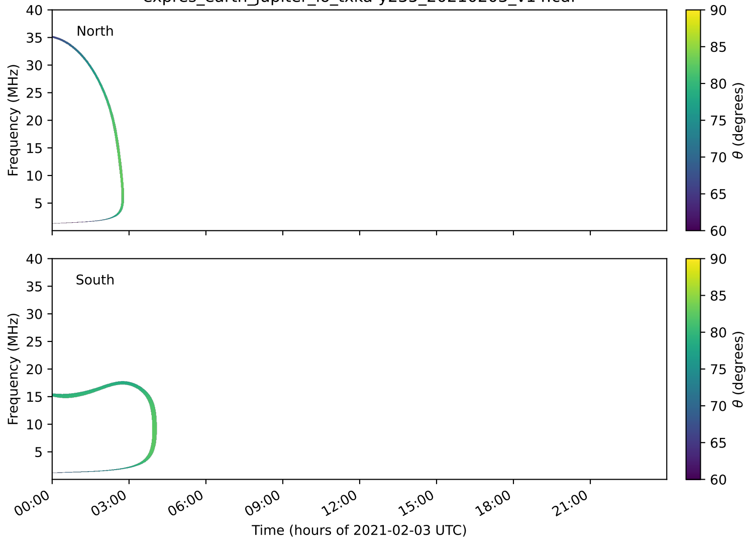
expres_earth_jupiter_io_txka-y235_20210203_v14.cdf
