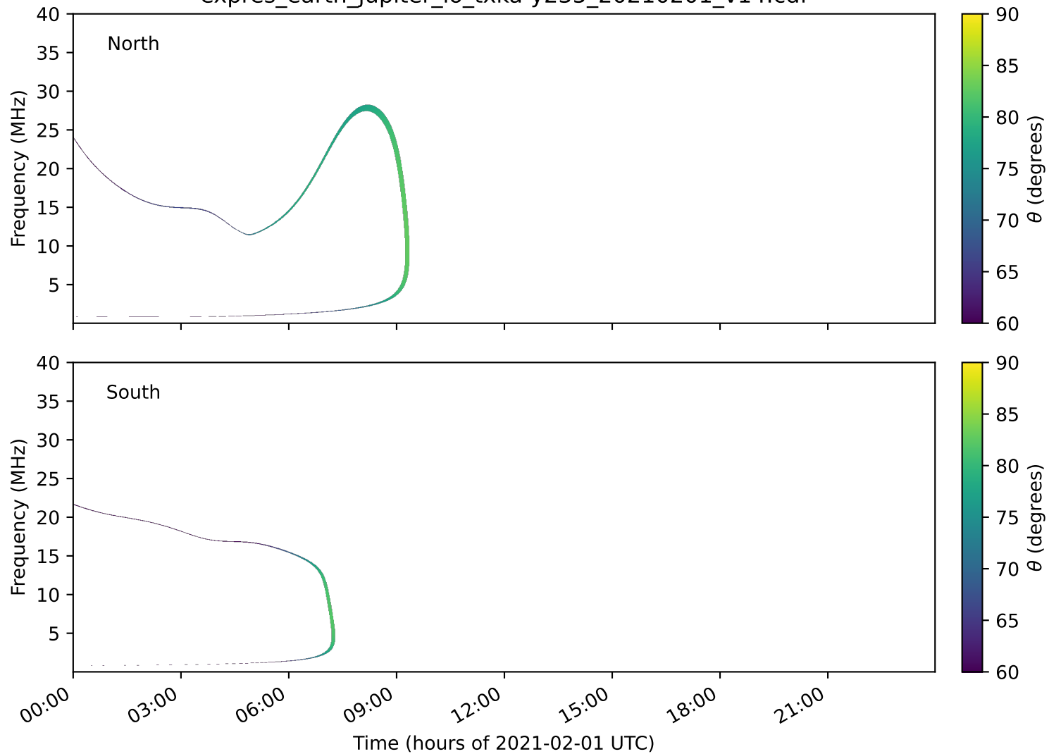
expres_earth_jupiter_io_txka-y235_20210201_v14.cdf
