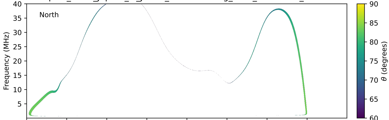
expres_earth_jupiter_io_jrm33_lossc-wid1deg_3kev_20210220_v11.cdf
