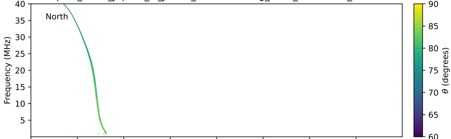
expres_earth_jupiter_io_jrm33_lossc-wid1deg_3kev_20210210_v11.cdf
