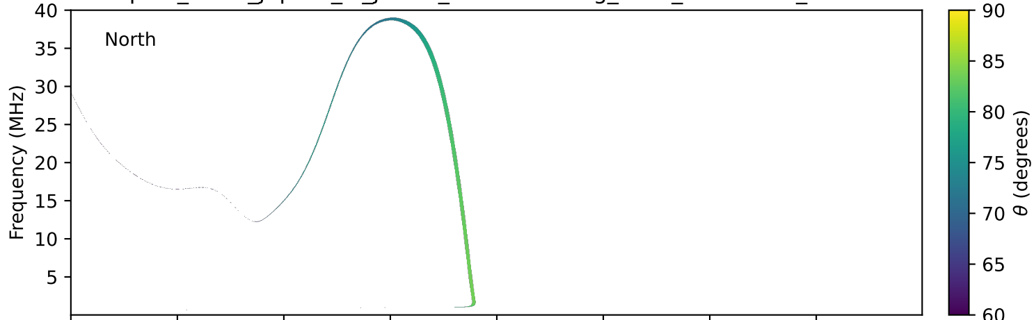
expres_earth_jupiter_io_jrm33_lossc-wid1deg_3kev_20210208_v11.cdf
