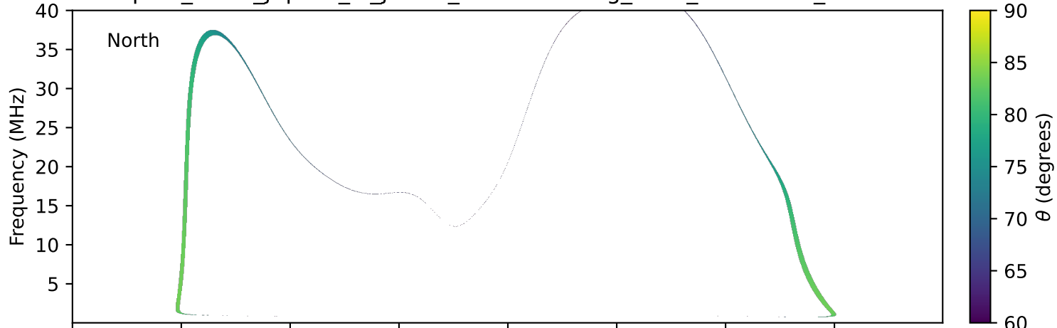
expres_earth_jupiter_io_jrm33_lossc-wid1deg_3kev_20210204_v11.cdf
