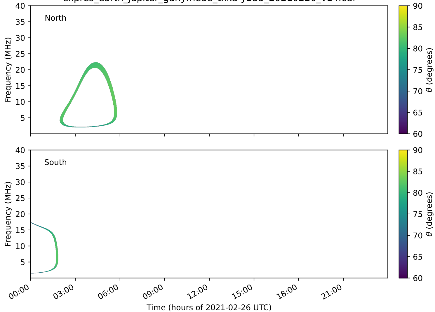
expres_earth_jupiter_ganymede_txka-y235_20210226_v14.cdf
