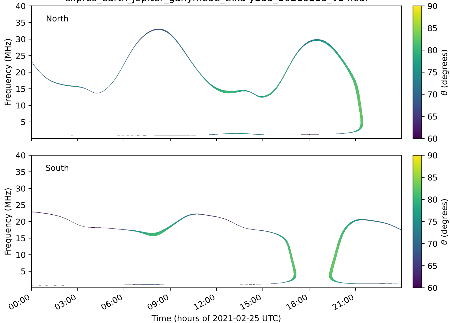
expres_earth_jupiter_ganymede_txka-y235_20210225_v14.cdf
