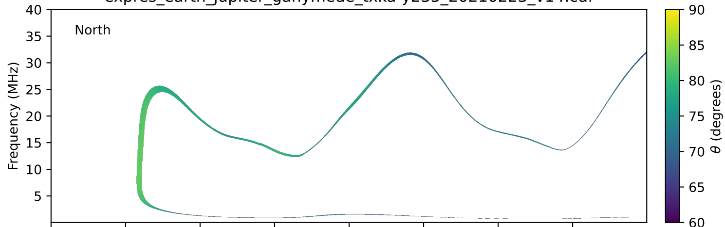
expres_earth_jupiter_ganymede_txka-y235_20210223_v14.cdf
