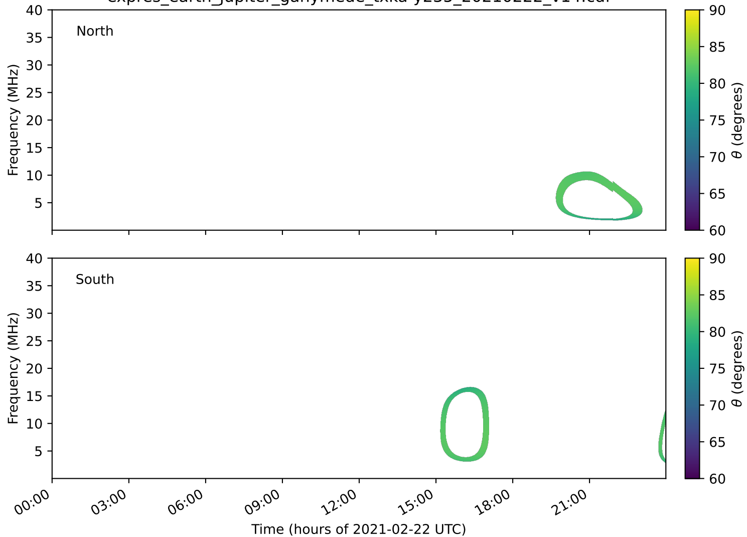
expres_earth_jupiter_ganymede_txka-y235_20210222_v14.cdf
