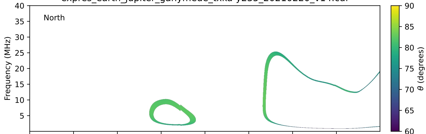
expres_earth_jupiter_ganymede_txka-y235_20210220_v14.cdf
