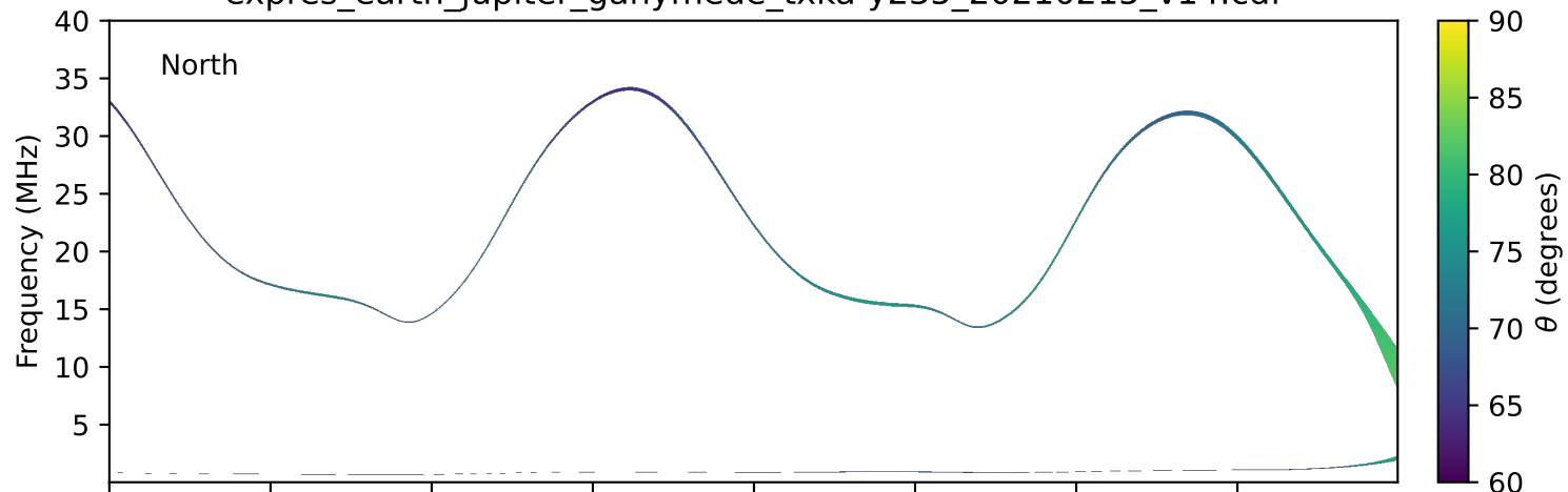
expres_earth_jupiter_ganymede_txka-y235_20210215_v14.cdf
