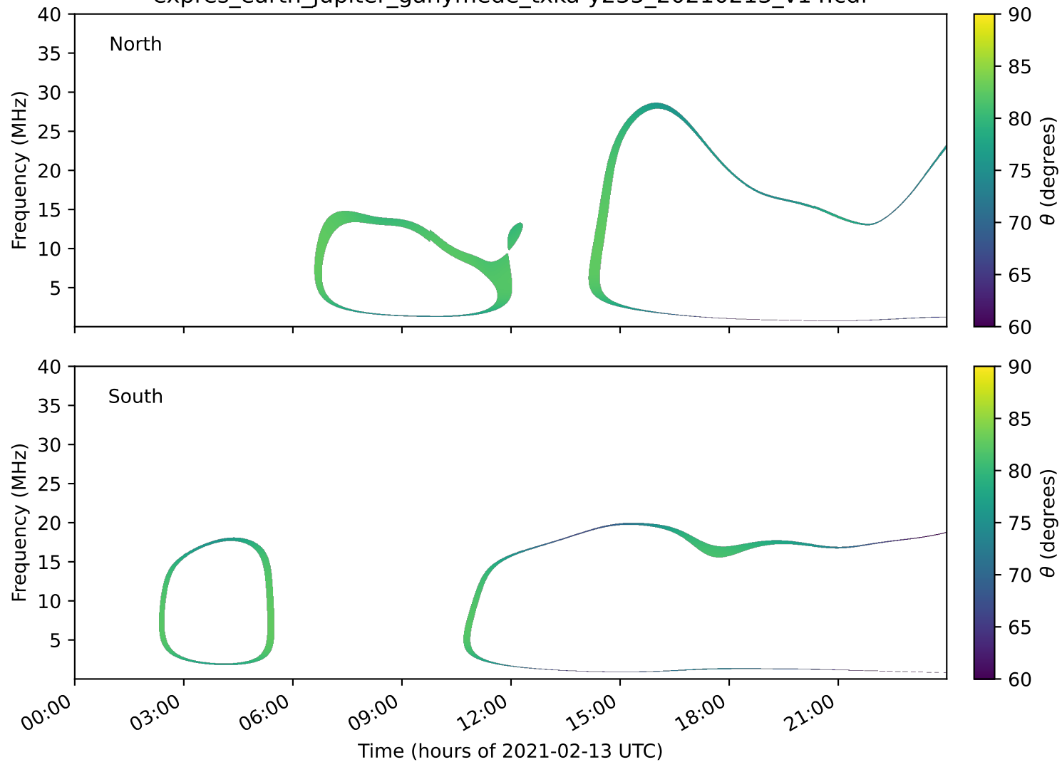
expres_earth_jupiter_ganymede_txka-y235_20210213_v14.cdf
