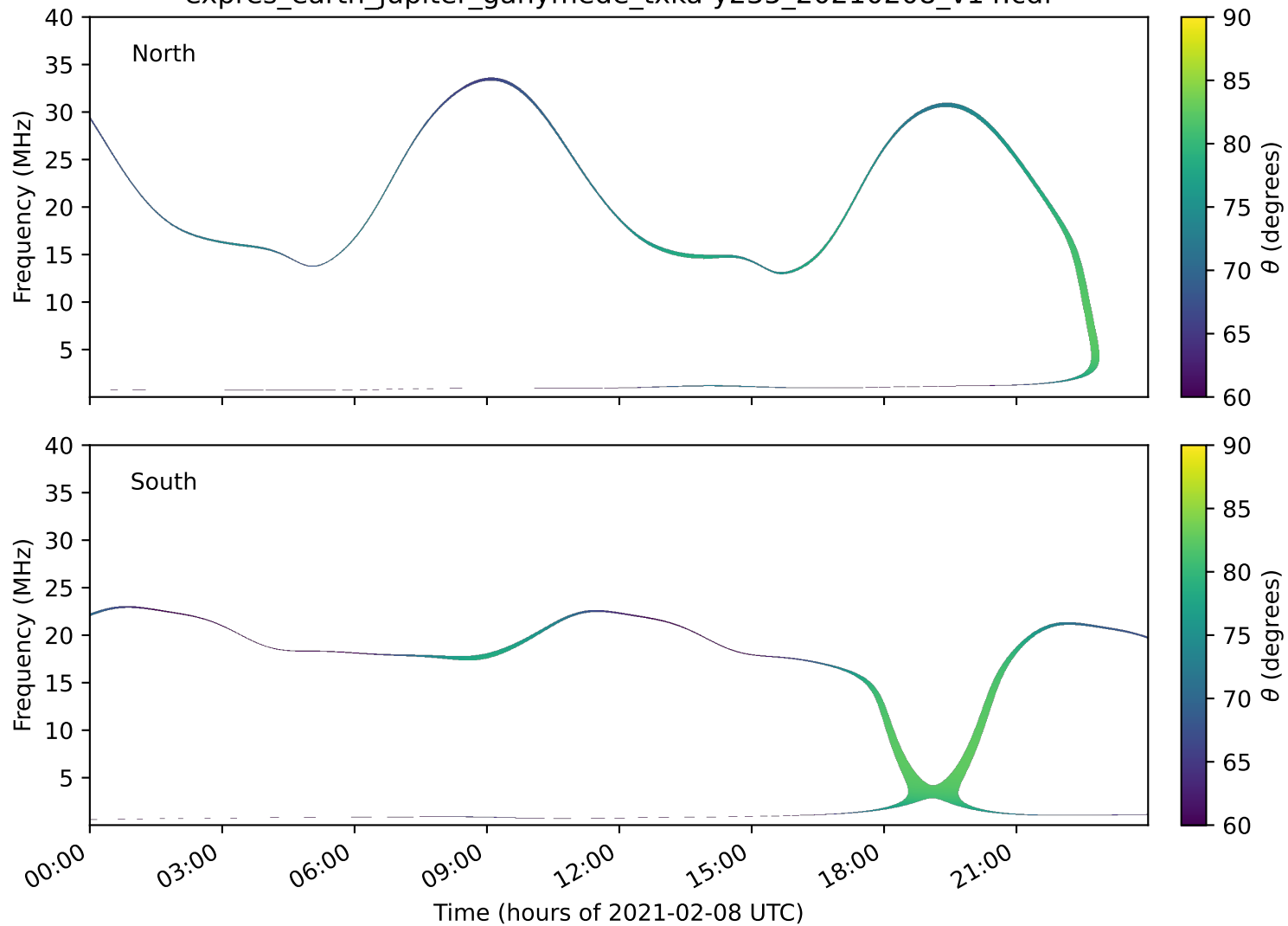
expres_earth_jupiter_ganymede_txka-y235_20210208_v14.cdf
