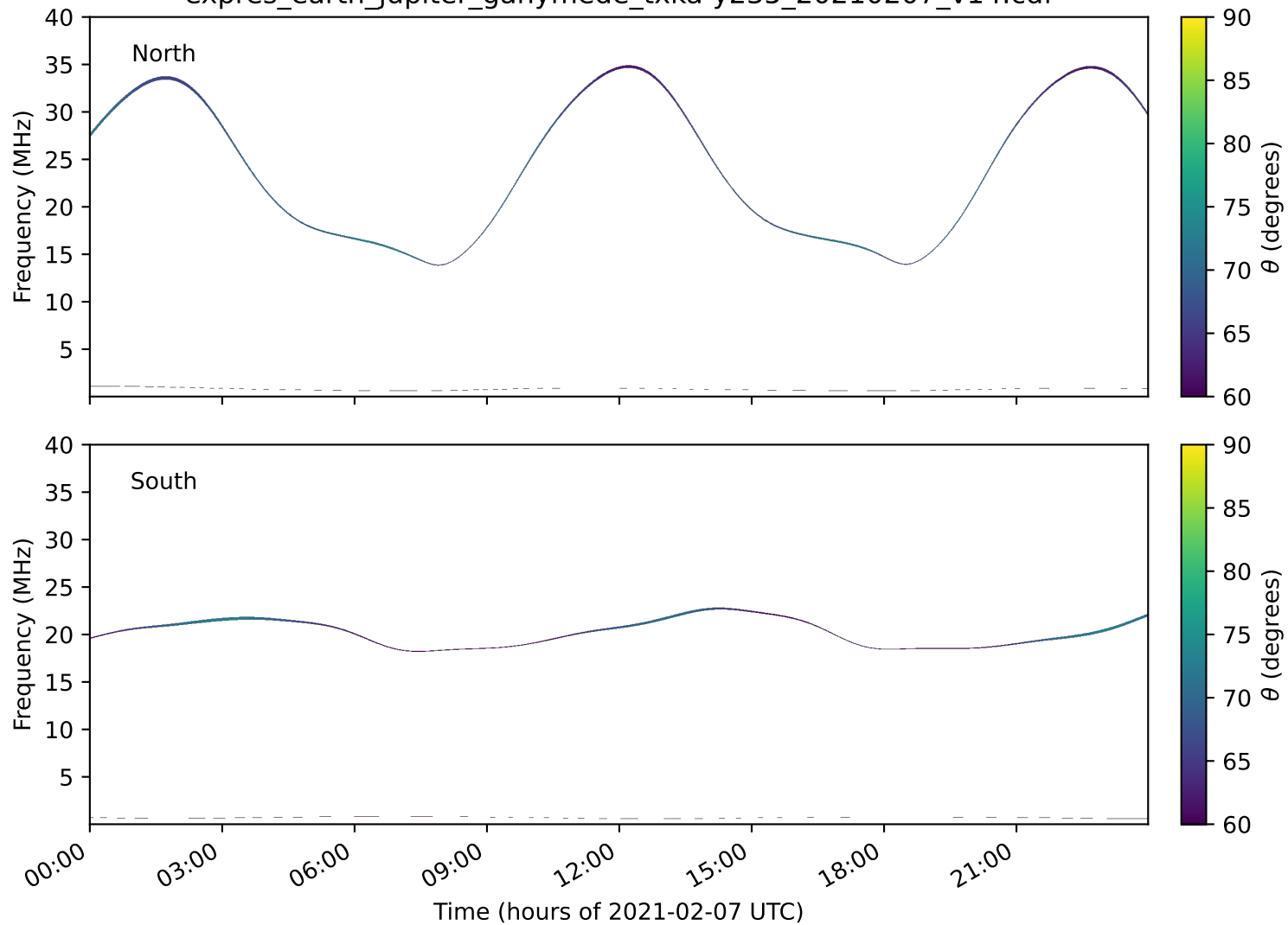
expres_earth_jupiter_ganymede_txka-y235_20210207_v14.cdf
