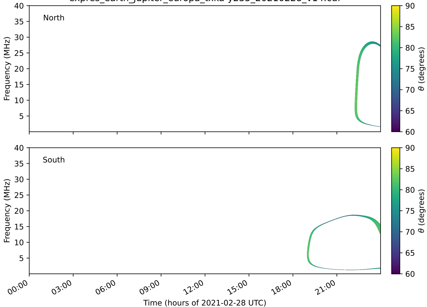
expres_earth_jupiter_europa_txka-y235_20210228_v14.cdf
