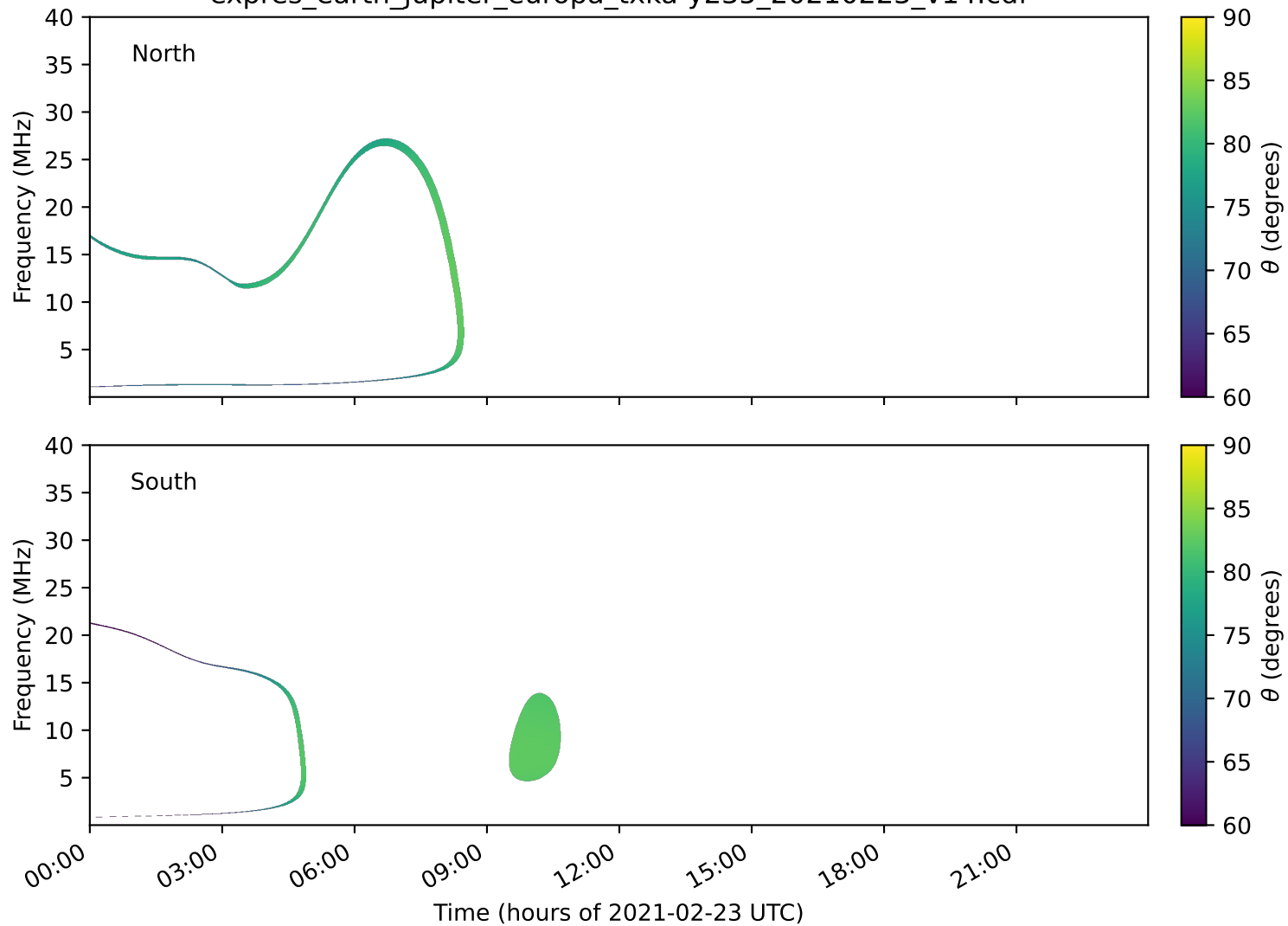
expres_earth_jupiter_europa_txka-y235_20210223_v14.cdf
