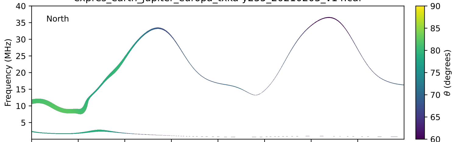
expres_earth_jupiter_europa_txka-y235_20210203_v14.cdf
