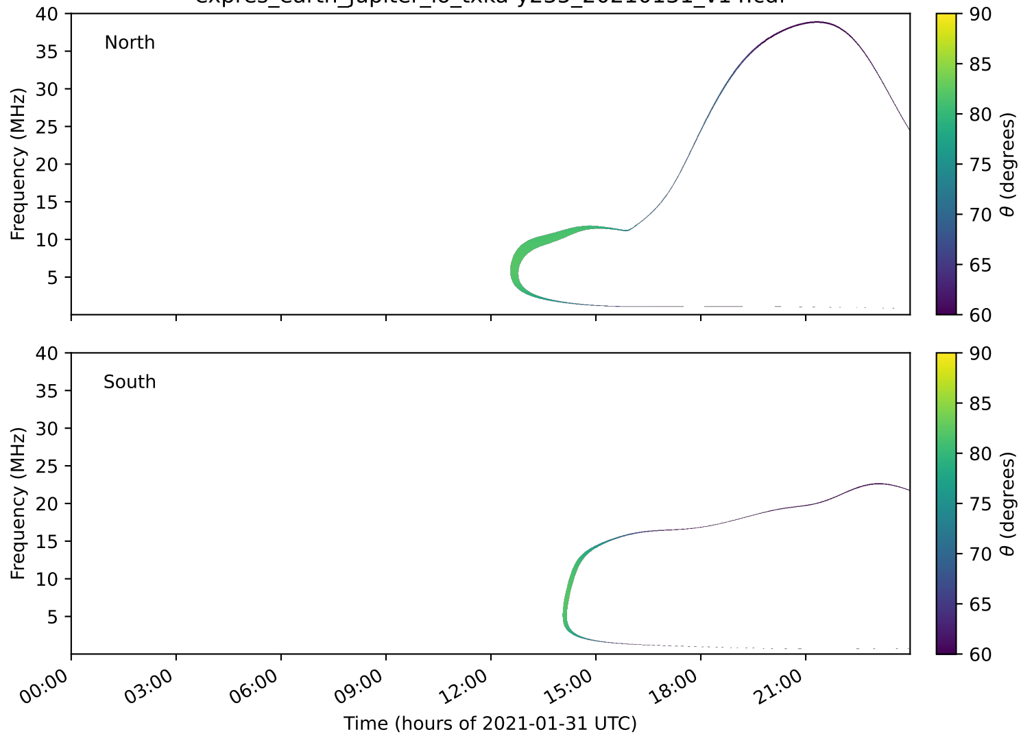
expres_earth_jupiter_io_txka-y235_20210131_v14.cdf
