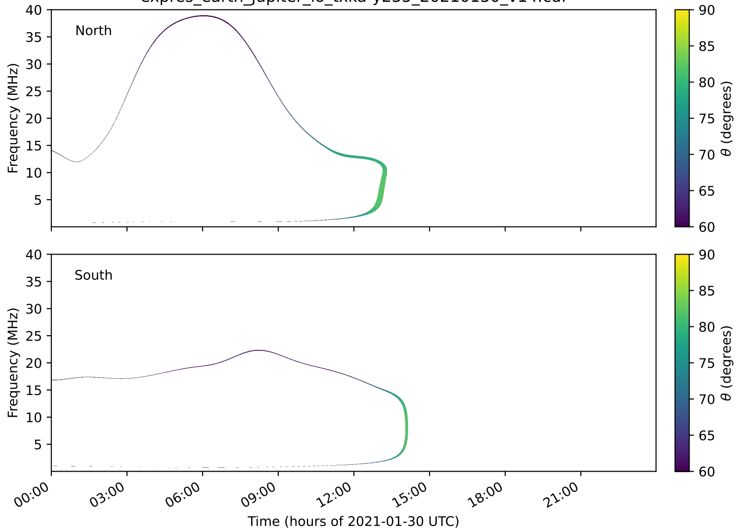
expres_earth_jupiter_io_txka-y235_20210130_v14.cdf
