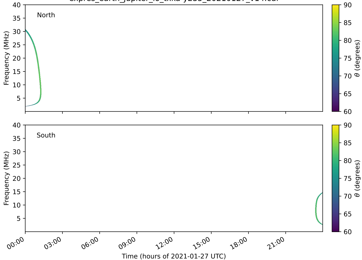
expres_earth_jupiter_io_txka-y235_20210127_v14.cdf
