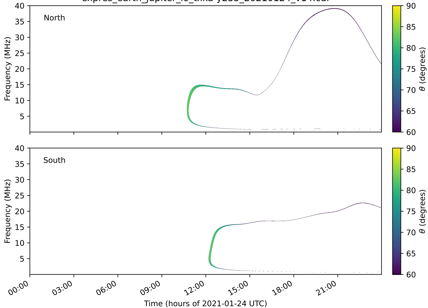
expres_earth_jupiter_io_txka-y235_20210124_v14.cdf
