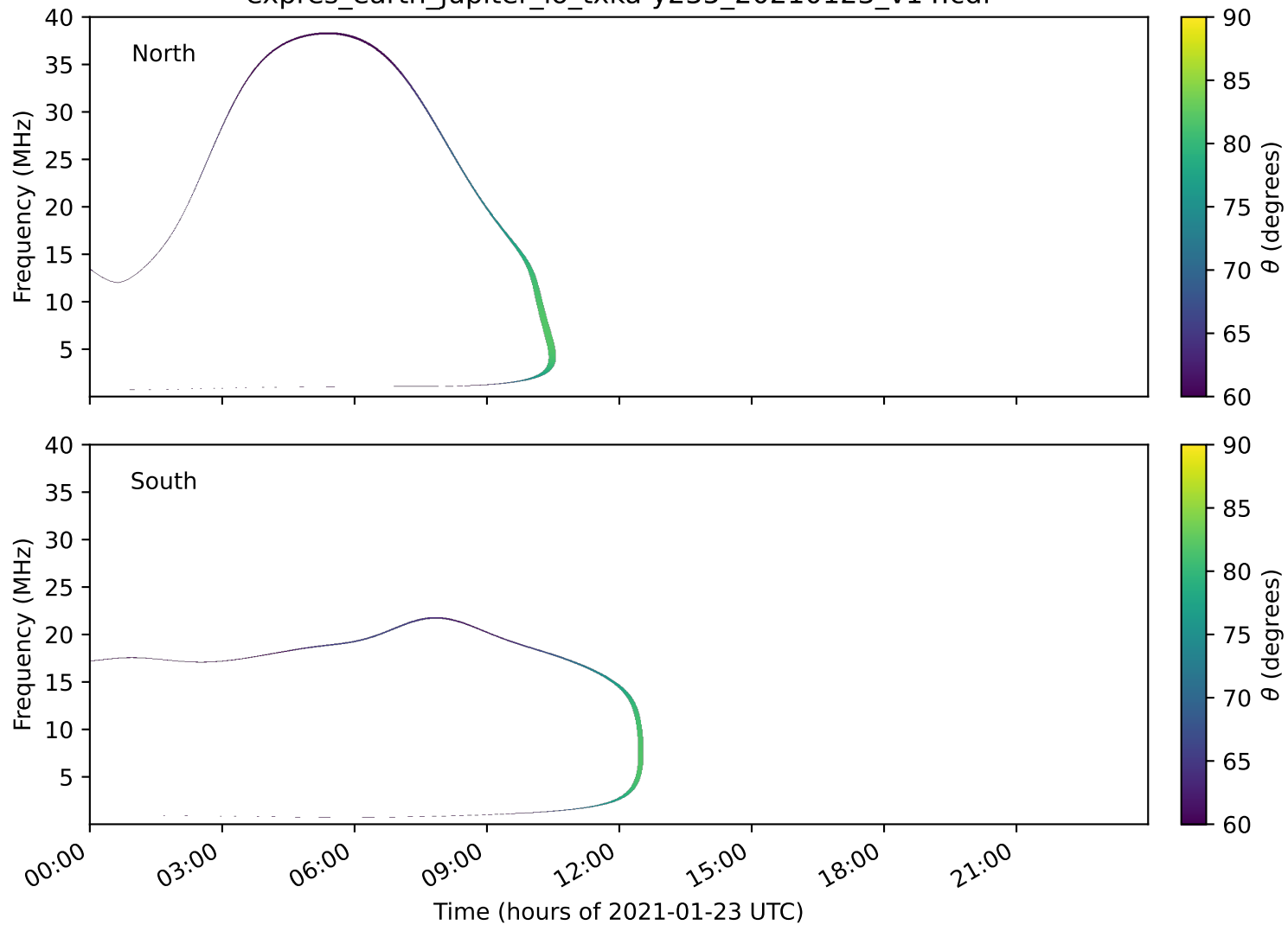
expres_earth_jupiter_io_txka-y235_20210123_v14.cdf
