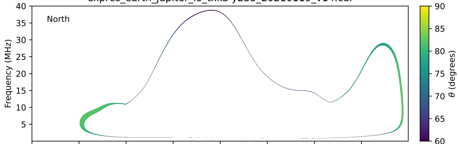
expres_earth_jupiter_io_txka-y235_20210119_v14.cdf
