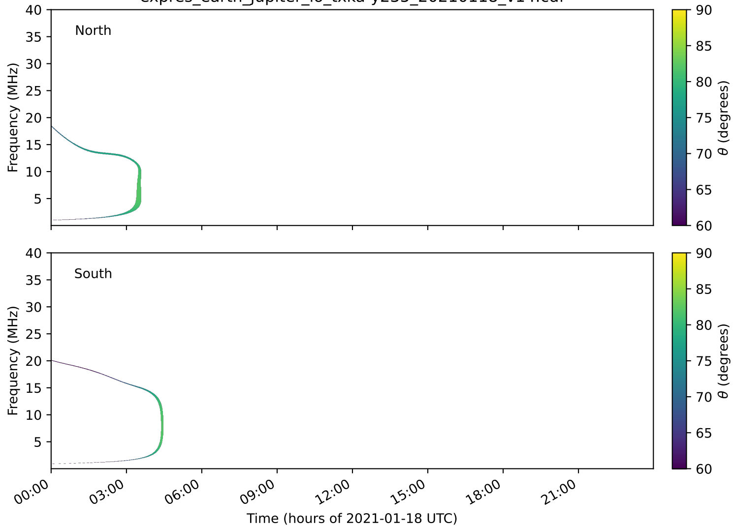
expres_earth_jupiter_io_txka-y235_20210118_v14.cdf
