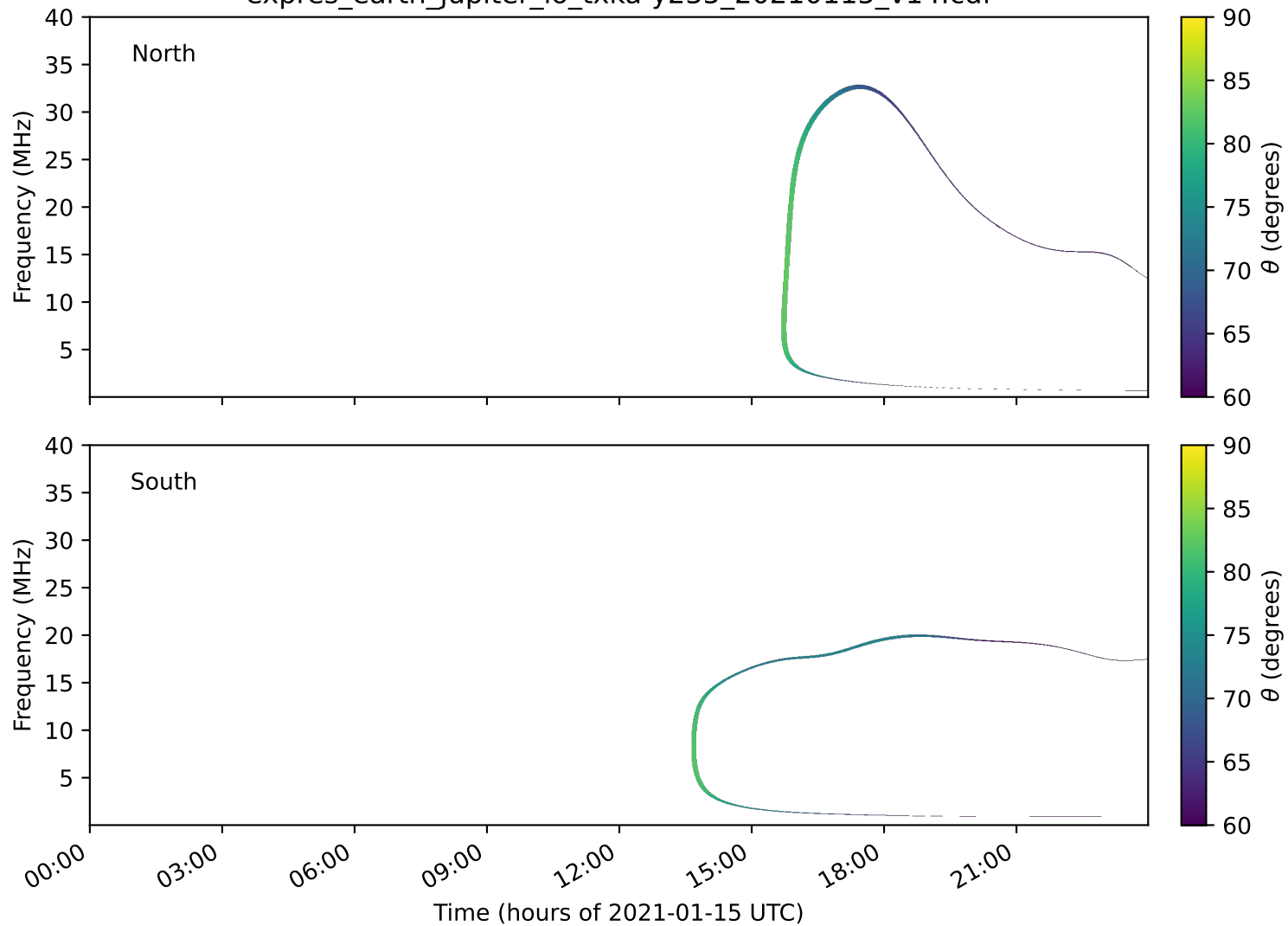
expres_earth_jupiter_io_txka-y235_20210115_v14.cdf
