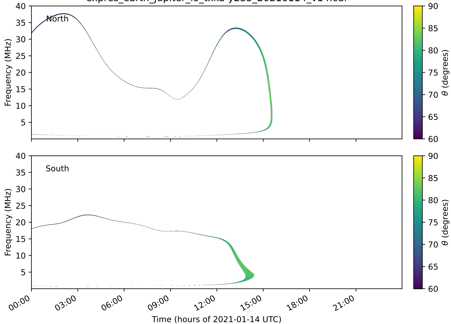
expres_earth_jupiter_io_txka-y235_20210114_v14.cdf
