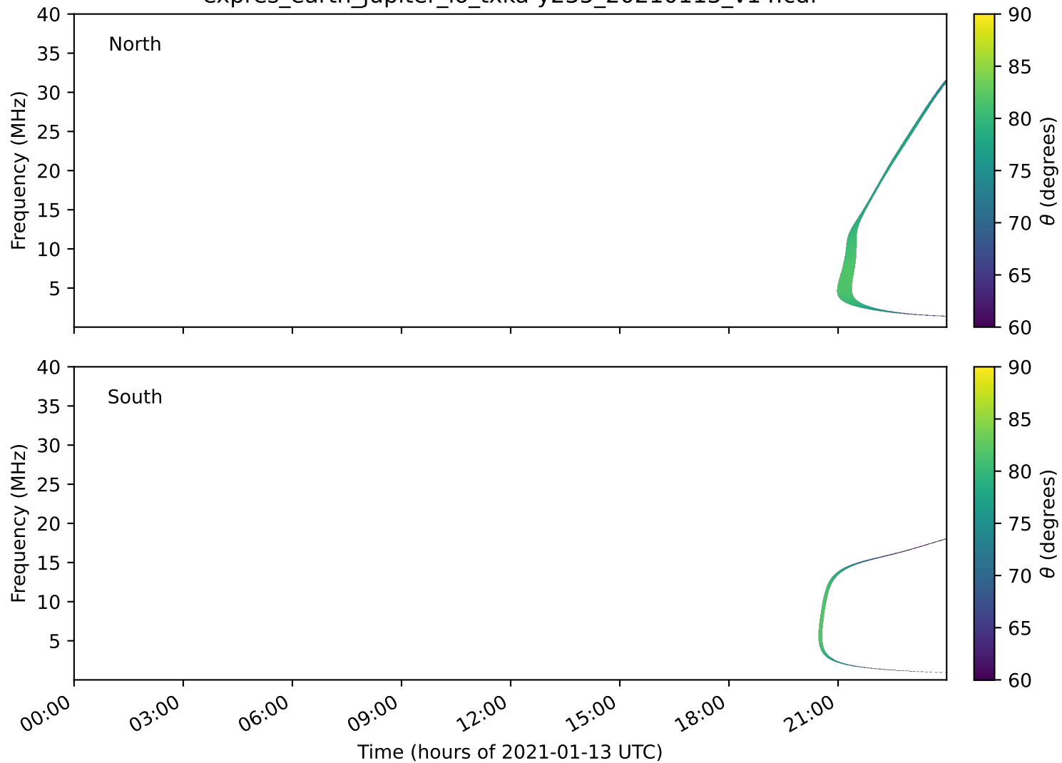
expres_earth_jupiter_io_txka-y235_20210113_v14.cdf
