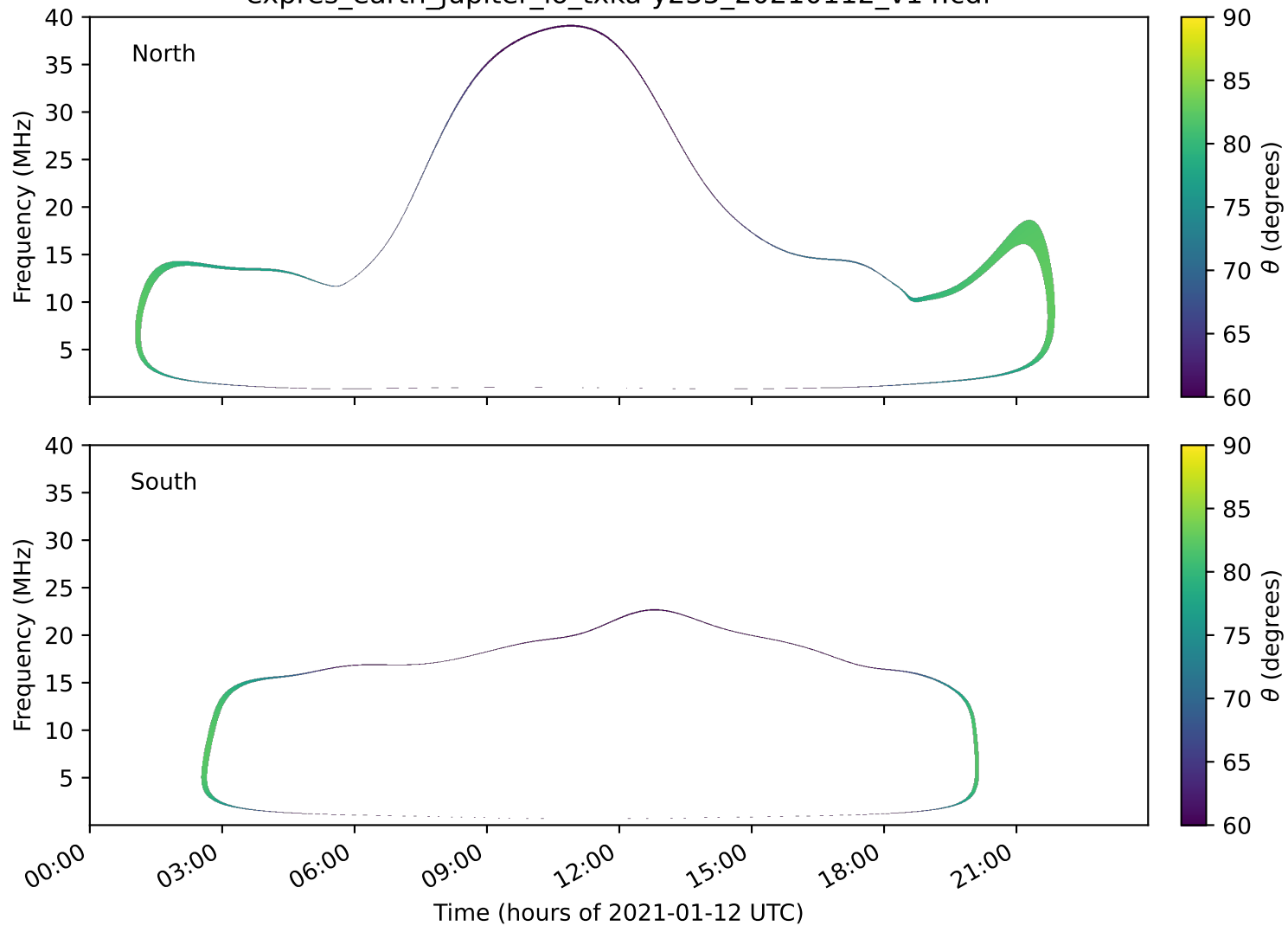
expres_earth_jupiter_io_txka-y235_20210112_v14.cdf
