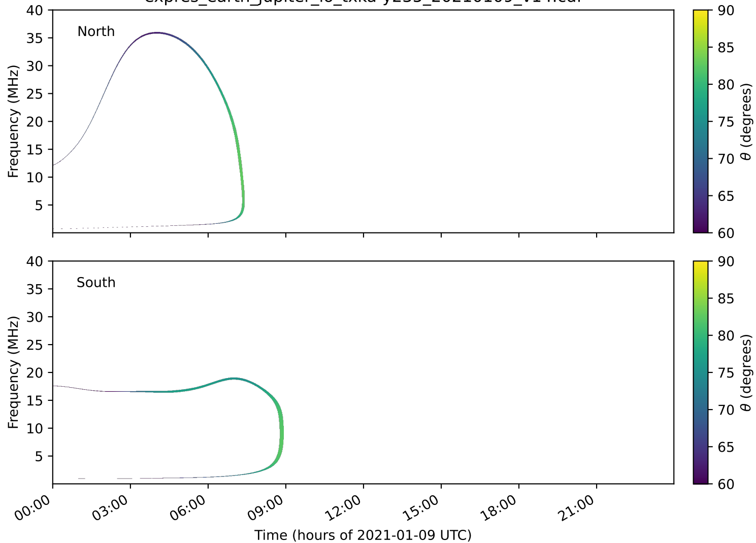
expres_earth_jupiter_io_txka-y235_20210109_v14.cdf
