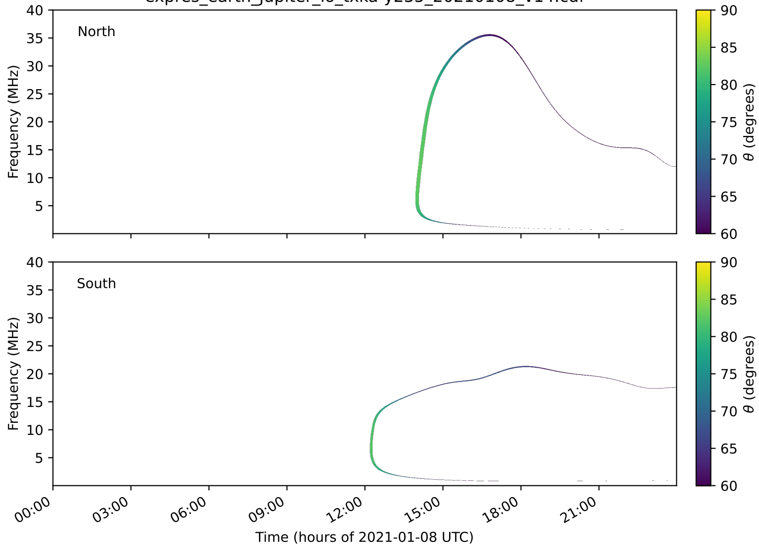
expres_earth_jupiter_io_txka-y235_20210108_v14.cdf
