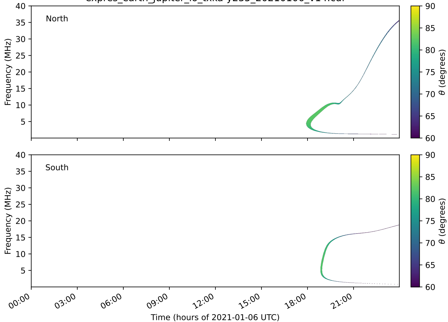
expres_earth_jupiter_io_txka-y235_20210106_v14.cdf
