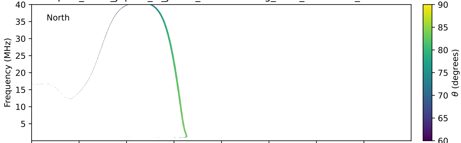
expres_earth_jupiter_io_jrm33_lossc-wid1deg_3kev_20210130_v11.cdf
