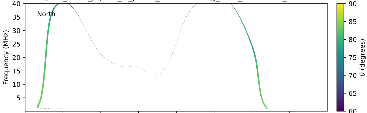
expres_earth_jupiter_io_jrm33_lossc-wid1deg_3kev_20210128_v11.cdf
